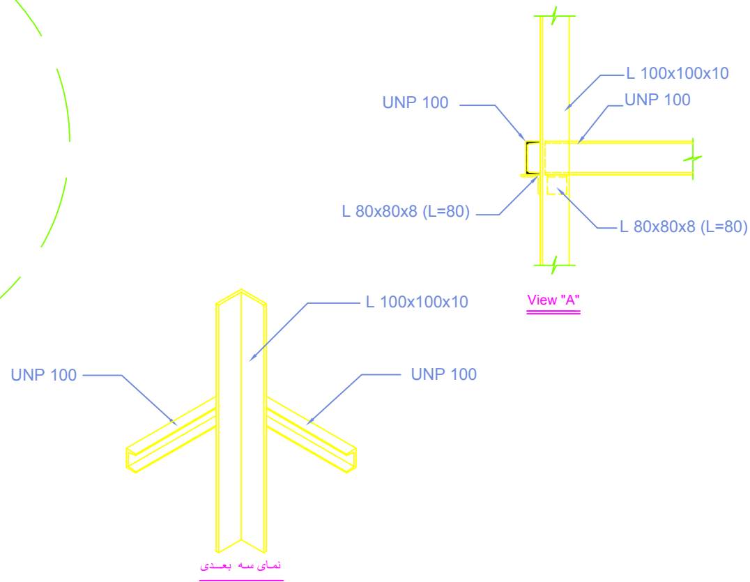
Detail ''A''
