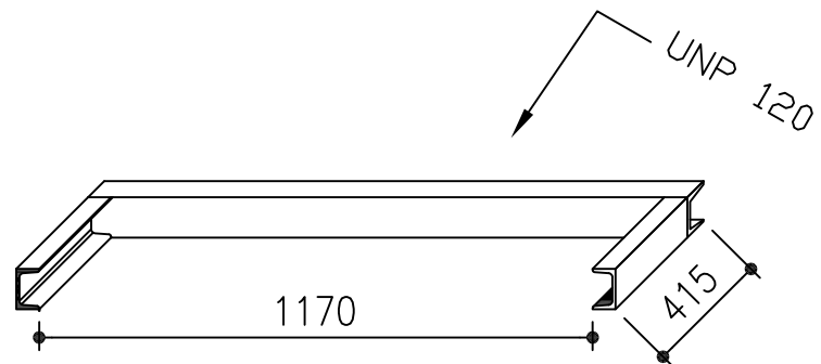
3D View Detail 'D'
