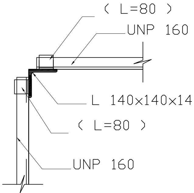
View "A"
